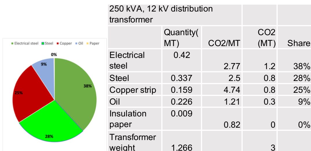
Fig. 8. Carbon footprint of a DT with Copper
