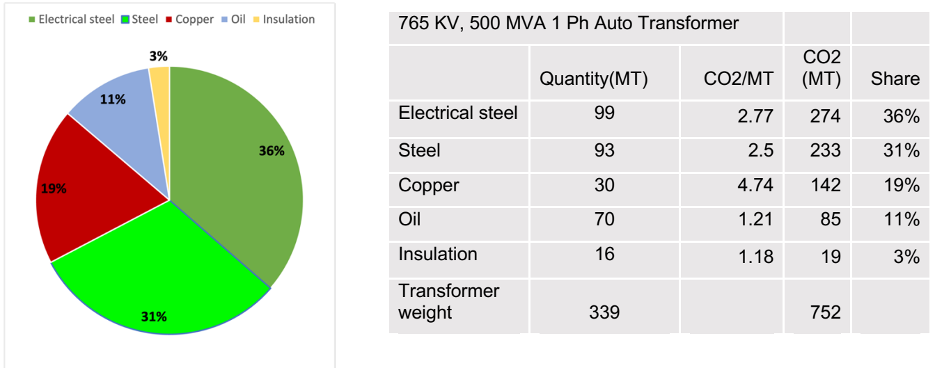
Fig. 6. Carbon footprint of an LPT
