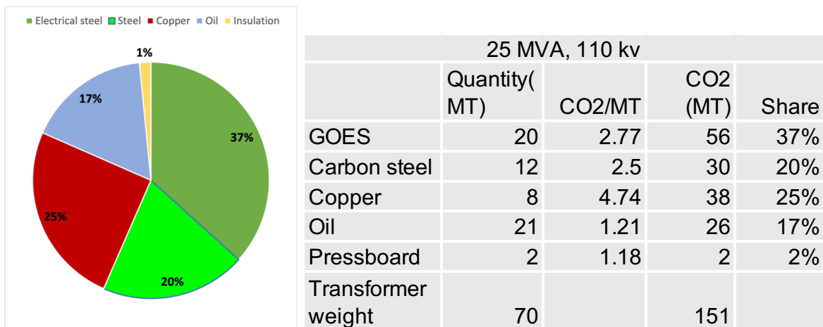
Fig. 7. Carbon footprint of an SPT
