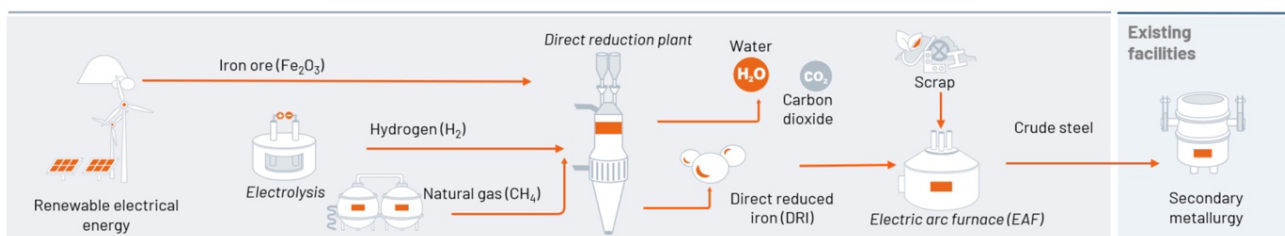
Fig. 3. Salcos steelmaking process of Salzgitter
