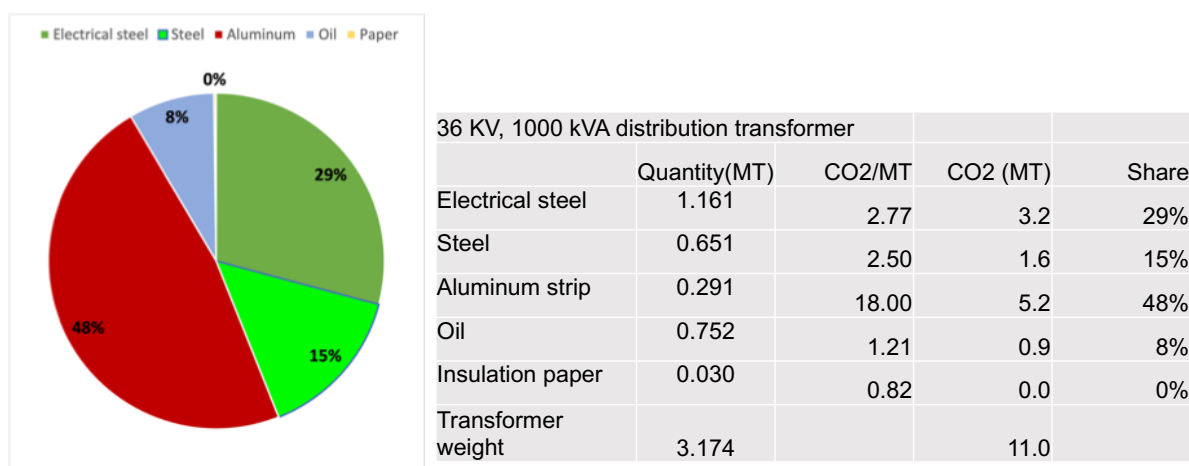
Fig. 9. Carbon footprint of a DT with Aluminium
